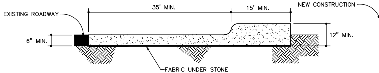
CROSS SECTION
