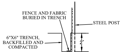
SECTION VIEW AT OPENING
