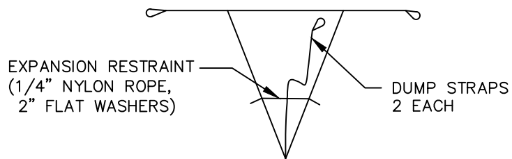
BAG DETAIL
