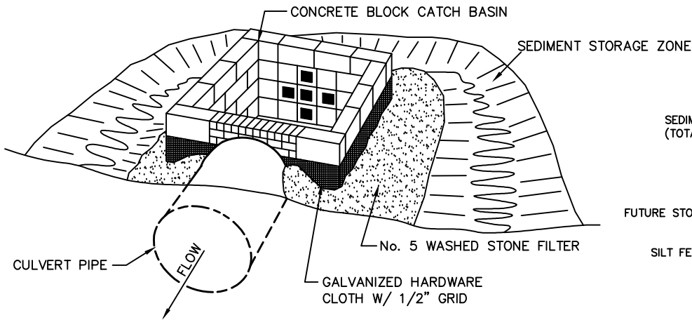
PERSPECTIVE VIEW
