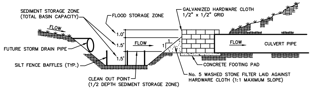
SECTION VIEW
