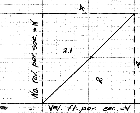
Rating Curve of K&E. Current Meter #362.
