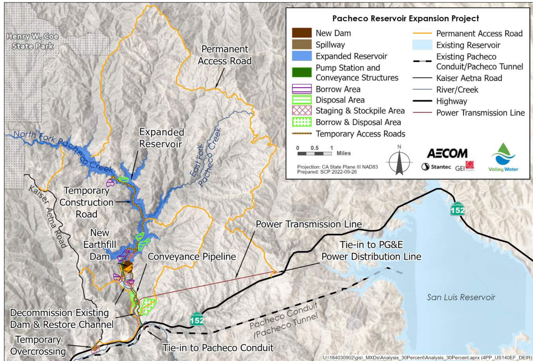
Figure 4-3. Temporary Roads and Borrow, Disposal, Staging, and Stockpiling Areas for the Staff Recommended Alternative
