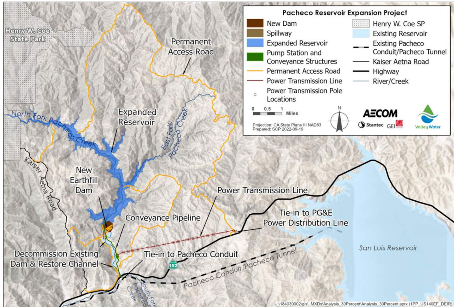
Figure ES-2. Permanent Facilities and Expanded Reservoir for Staff Recommended Alternative
