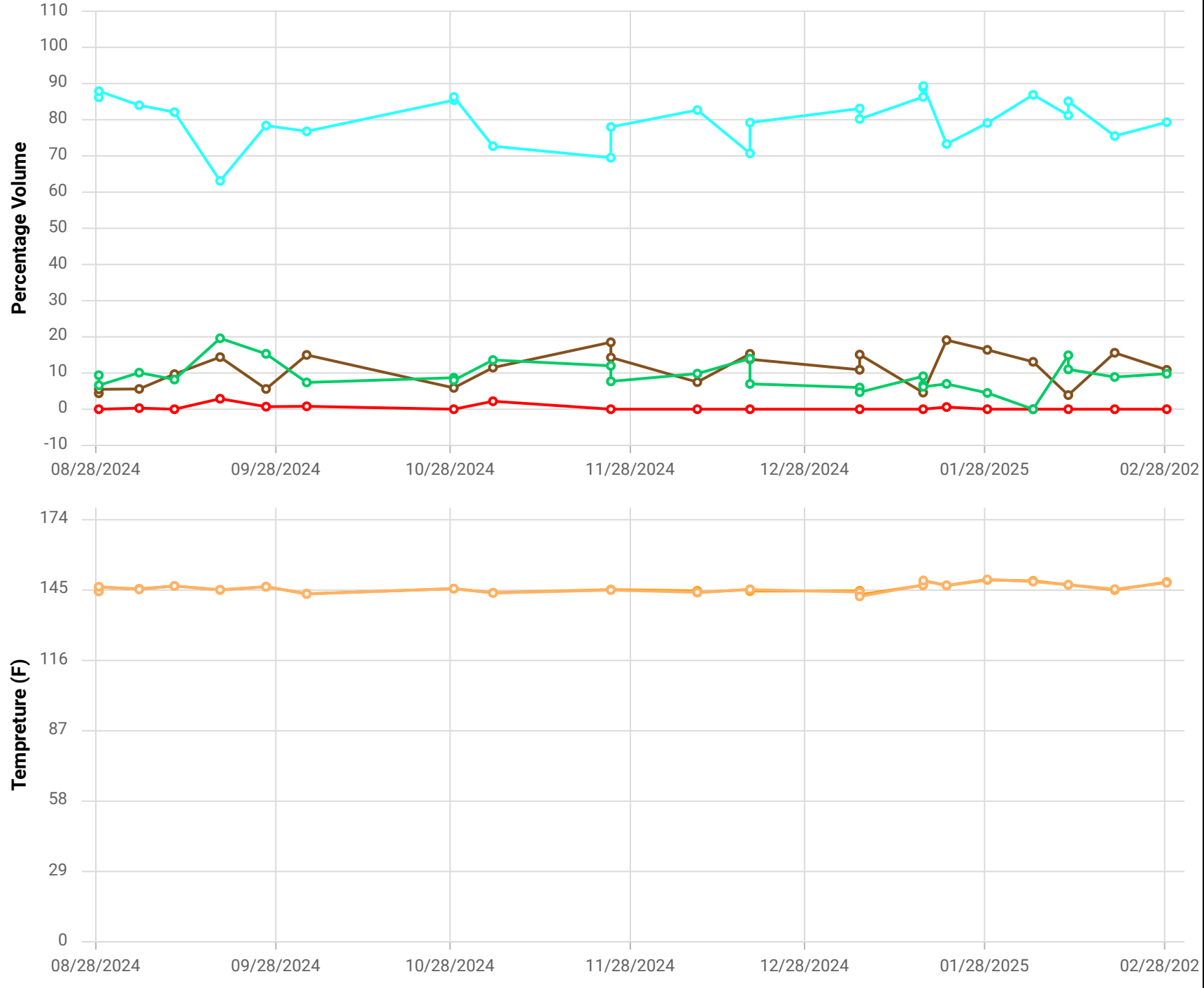
Chiquita Canyon Landfill Parameter Chart: Multiscale Date Range: 08/28/2024 - 02/28/2025 Chart generation date: 3/7/25
