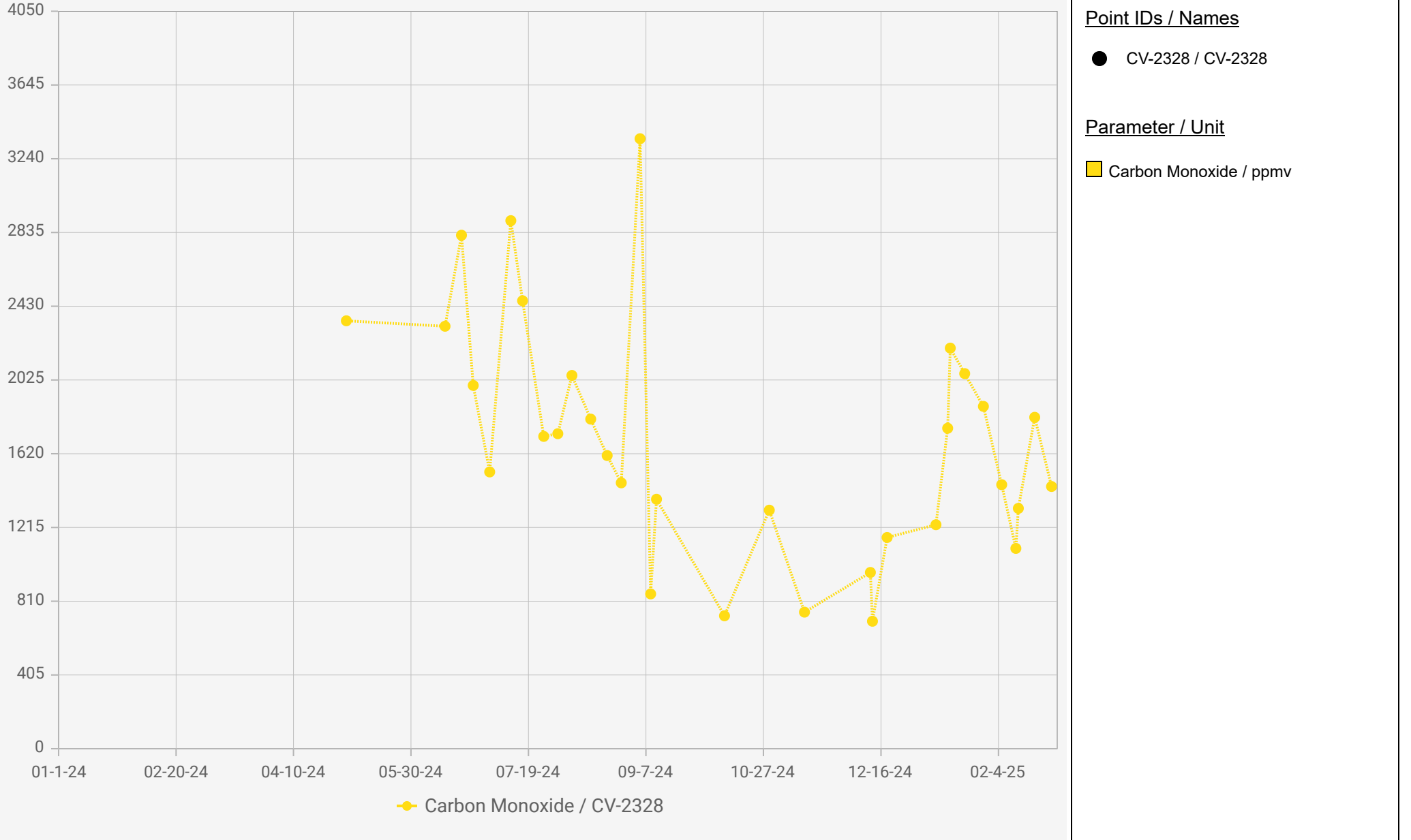
Chiquita Canyon Landfill - LAB DATA Points Chart Date Range : 01/01/2024 to 02/28/2025 Chart generation date : 03/07/2025
